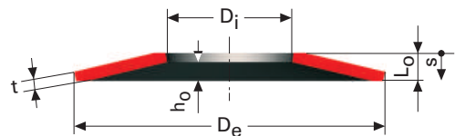
Group 3 springs
